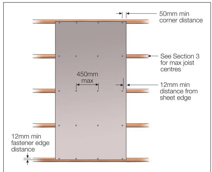
FIGURE 2 FIXING REQUIREMENTS
