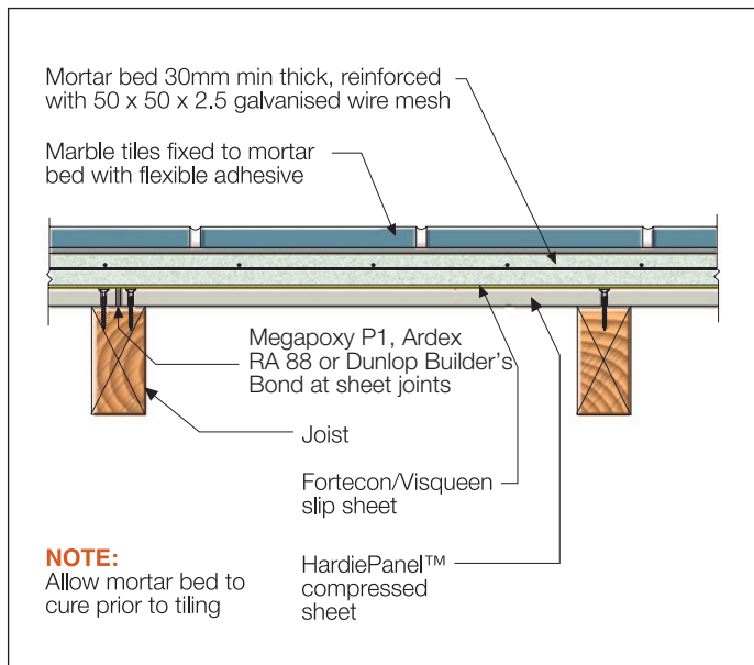
FIGURE 17 MORTAR BED
