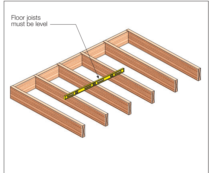
FIGURE 1 JOIST LAYOUT
