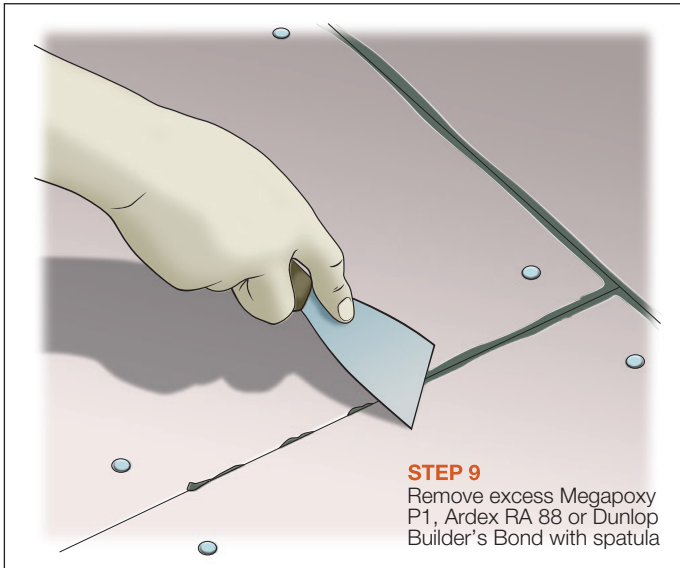
FIGURE 12 REMOVE EXCESS EPOXY
